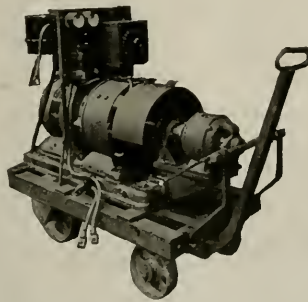
TYPE OF SINGLE-OPERATOR ELECTRIC WELDING OUTFIT
